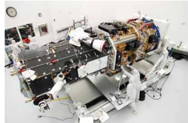
WorldView-2 – BCP 5000
