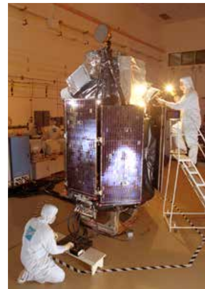
QuickBird – BCP 2000
